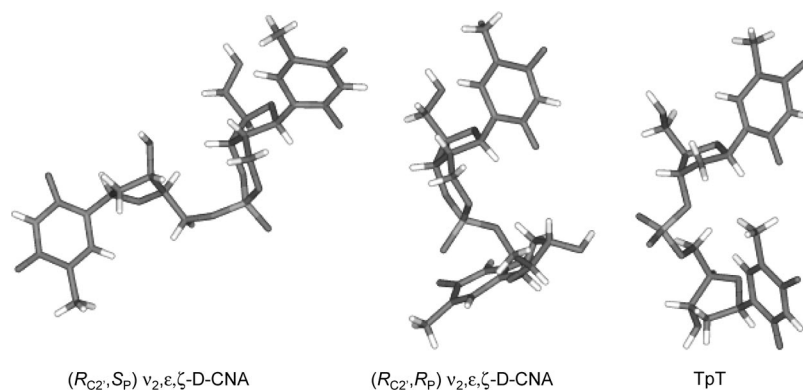
Figure 5. Tentative model of the conformation of the (R_{C2'}, S_P) and (R_{C2'}, R_P) v_{2,\epsilon,\zeta} -D-CNA diastereoisomers derived from the NMR spectroscopic data and that of TpT. [36]
