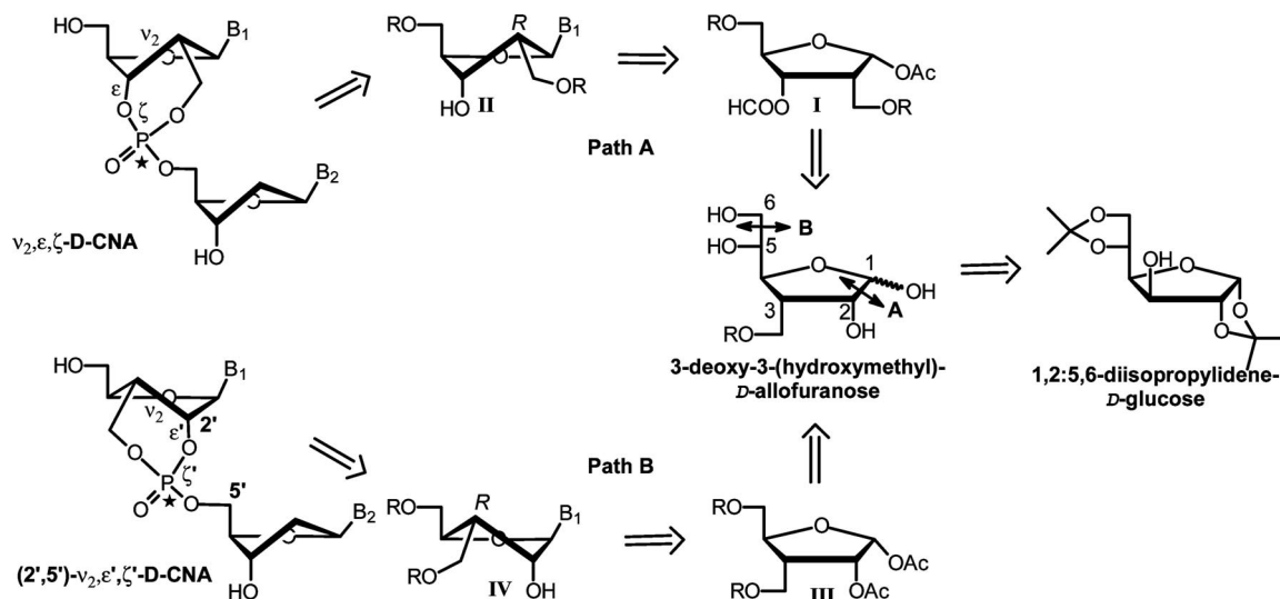
Figure 2. Retrosynthetic pathway for the synthesis of v_2, \epsilon, \zeta -D-CNA dimers and their (2',5')\text{-}v_2, \epsilon', \zeta' -D-CNA analogues from common intermediate 3-deoxy-3-(hydroxymethyl)-D-allofuranose.
