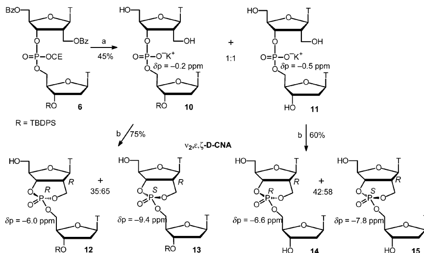
Scheme 3. Reagents and conditions: (a) K 2 CO 3 , MeOH/H 2 O (4:1), room temp., 6 h; (b) 1-(mesitylene-2-sulfonyl)-3-nitro-1,2,4-triazole (MSNT), pyridine, room temp. for 1 h, then 80 °C for 30 min, and 90 °C for 30 min.
