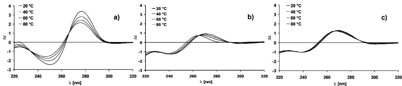
Figure 3. CD spectra in 10 mM sodium phosphate (pH 7.0) at 80, 60, 40, and 20 °C of: (a) T p T; (b) ( R C2' , R P ) \nu_2, \epsilon, \zeta -D-CNA TT 14 ; and (c) ( R C2' , S P ) \nu_2, \epsilon, \zeta -D-CNA TT 15 .
