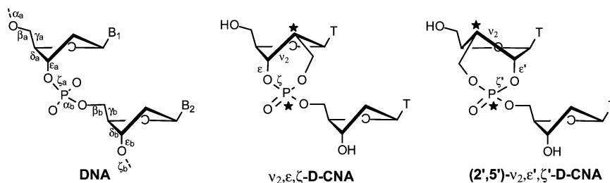
Figure 1. Left: the six backbone torsion angles (labeled \alpha_a to \zeta_a for the upper nucleotide and \alpha_b to \zeta_b for the lower nucleotide) of nucleic acids; middle: v_2, \epsilon, \zeta -D-CNA dinucleotide, in which v_2, \epsilon, \zeta are stereocontrolled to canonical or noncanonical values by a dioxaphosphorinane ring structure exhibiting two new asymmetric centers; right: (2',5')\text{-}v_2, \epsilon', \zeta' -D-CNA dinucleotide, in which v_2, \epsilon', \zeta' are stereocontrolled by a dioxaphosphorinane ring structure exhibiting an asymmetric phosphorus center.
