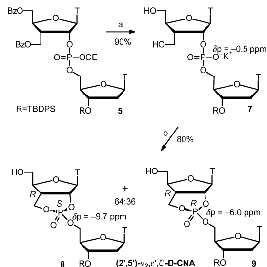
Scheme 2. Reagents and conditions: (a) \text{K}_2\text{CO}_3 , \text{MeOH}/\text{H}_2\text{O} (4:1), room temp., 6 h; (b) 1-(mesitylene-2-sulfonyl)-3-nitro-1,2,4-triazole (MSNT), pyridine, room temp. for 1 h, then 80 °C for 30 min, and 90 °C for 30 min.
