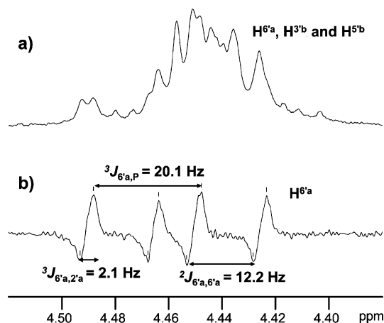
Figure 4. NMR spectroscopic data for 6'-b-H of (R_{C2'}, R_P) v_{2,\epsilon,\zeta} -D-CNA TT 14 : (a) ^1\text{H} NMR and (b) ^1\text{H} COSY with selective irradiation at \delta = 2.89 ppm.
