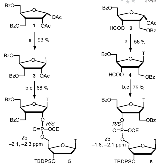
Scheme 1. Reagents and conditions: (a) TMSOTf, bis(trimethylsilyl)thymine, \text{CH}_3\text{CN} , reflux, 2 h; (b) concentrated \text{NH}_4\text{OH} , room temp., 2 h; (c) 3'-O- tert -butyldiphenylsilylthymidine-5'-O-phosphoramidite (2 equiv.), tetrazole (10 equiv.), \text{CH}_3\text{CN} then collidine, \text{I}_2/\text{H}_2\text{O} , room temp., 3 h.
